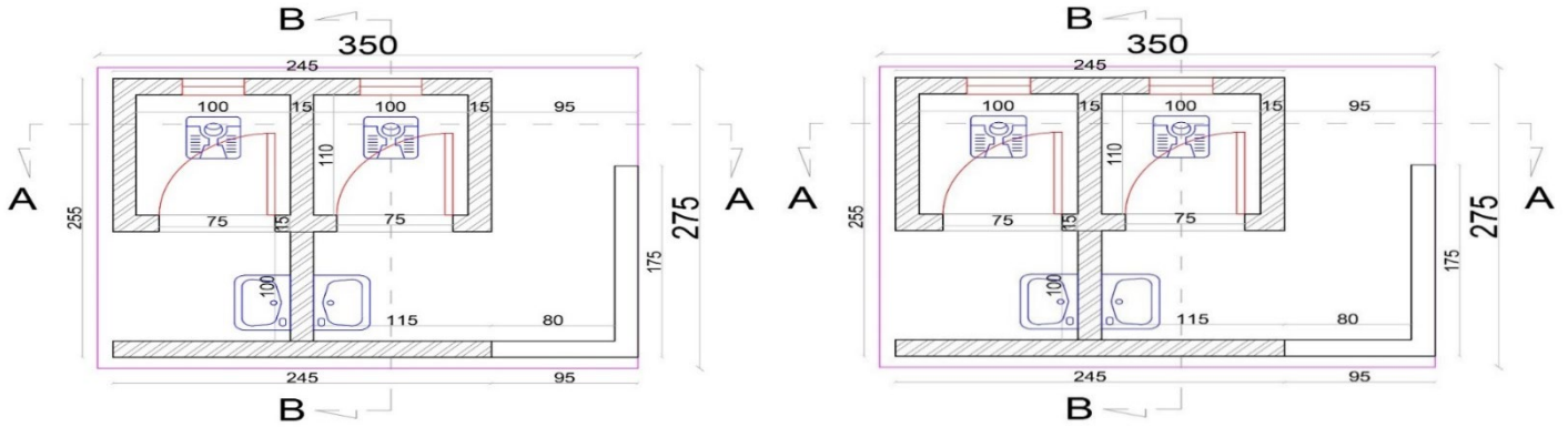
plan for latrine 2 cells
