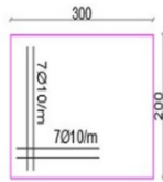
SLAB OF SEPTIC TANK
